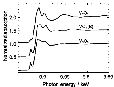
Figure 5. Vanadium K edge XANES spectra of anosovite-type V_3O_5 , VO_2(B) , and V_2O_3 with corundum structure.
