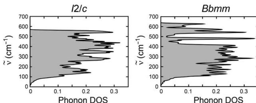
Figure 8. Phonon density of states of the high-temperature polymorph ( I2/c ) and the anosovite-type ( Bbmm ) V_3O_5 .
